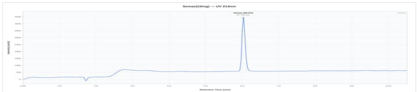
Semax 10mg - SMX-A701: UV Chromatogram
