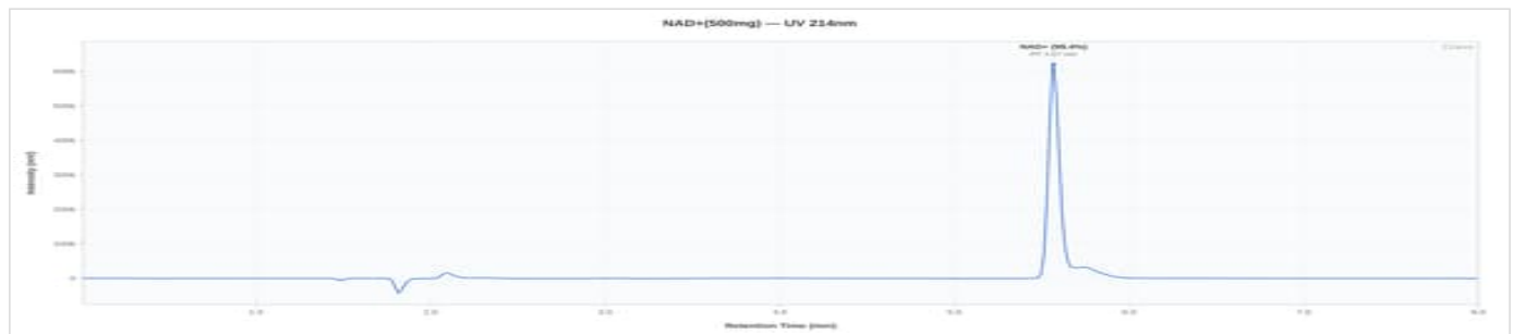
NAD+ 500mg - NAD-A463: UV Chromatogram
