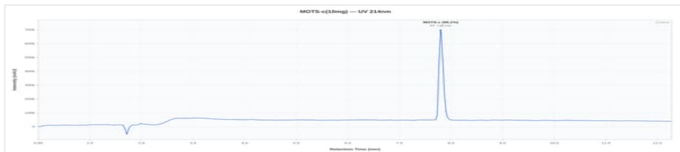
MOTS-C 10mg - MTC-A274: UV Chromatogram
