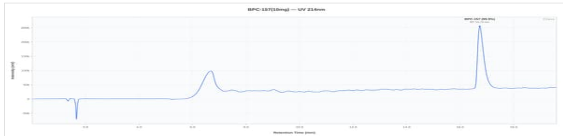
BPC-157 10mg - BPC-A319: UV Chromatogram
